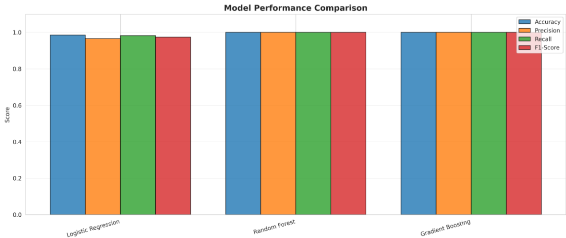
Figure 4: Model Performance Comparison
