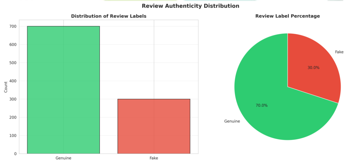
Figure 6: Review Label Distribution
