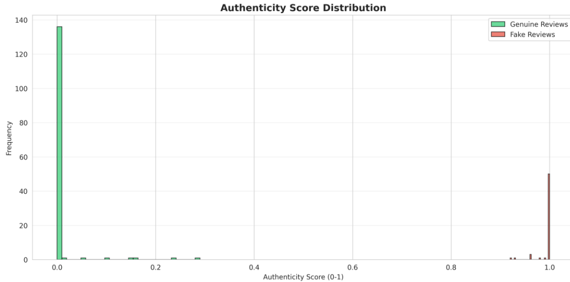
Figure 3: Authenticity Score Distribution
