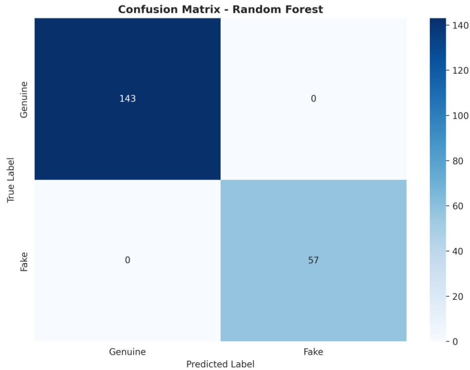
Figure 5: Confusion Matrix (Random Forest)
