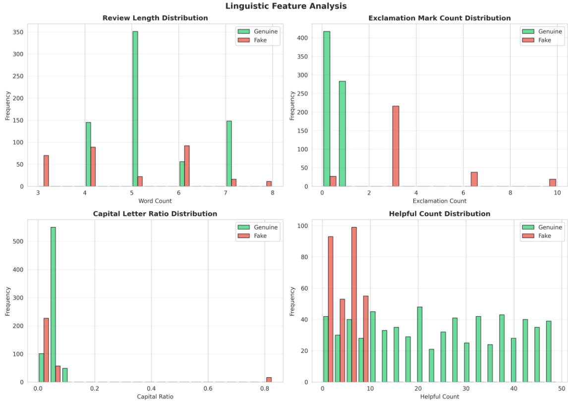
Figure 1: Linguistic Feature Analysis by Review Type
